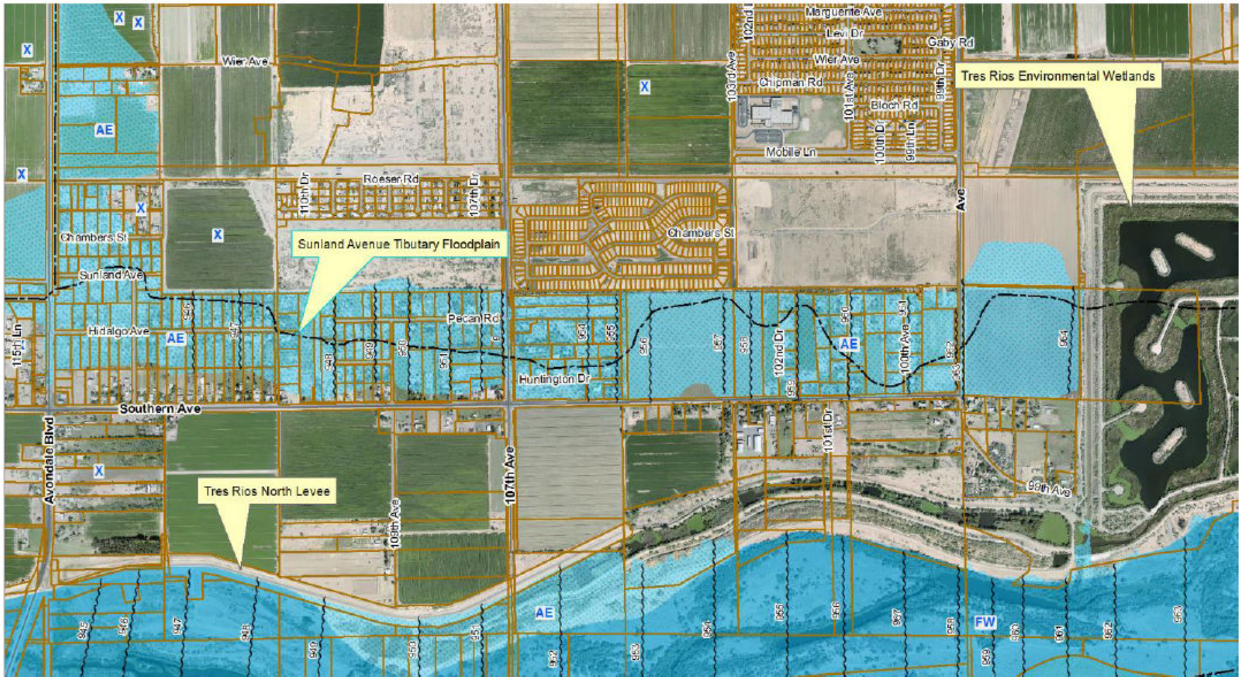
Figure 1 – Sunland Avenue Tributary Floodplain
